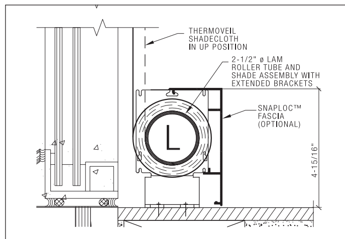
Detail SAL = Sill/LAM™/SnapLoc™ Fascia (Optional)
