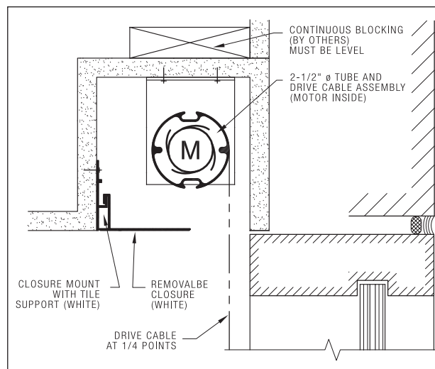
Detail HPM = Head/Pocket/Motor
