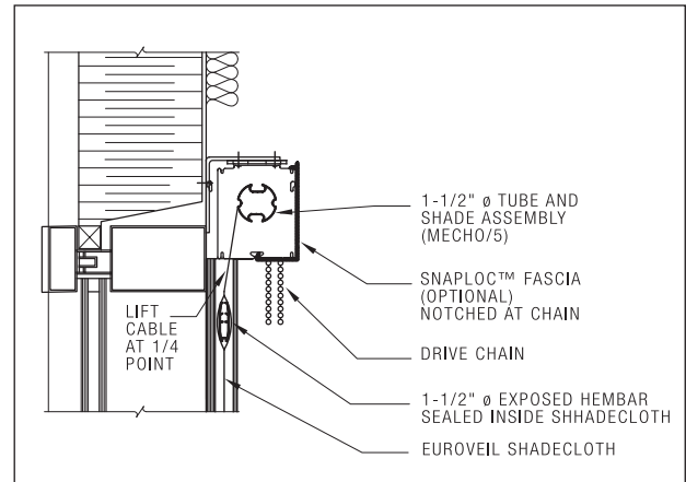
Detail HB = Head/Bracket/SnapLoc™ Fascia (Optional)
