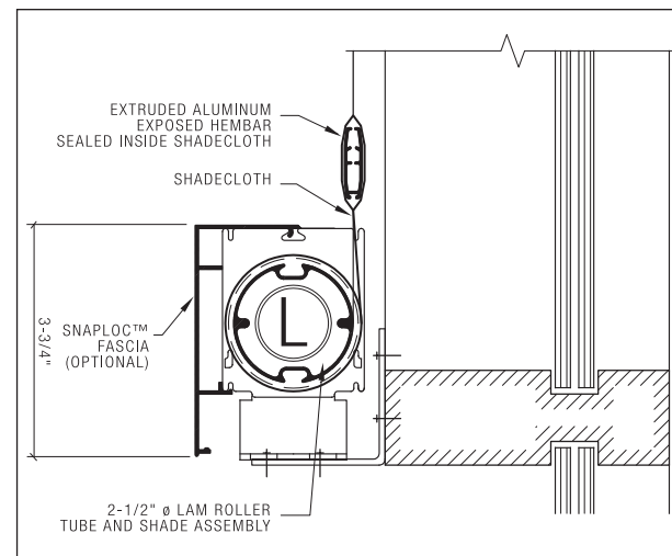
Detail SAL = Sill/LAM™/SnapLoc™ Fascia (Optional)
