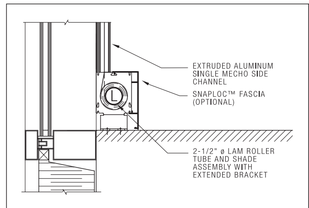
Detail SAL = Sill/LAM™/SnapLoc™ Fascia (Optional)
